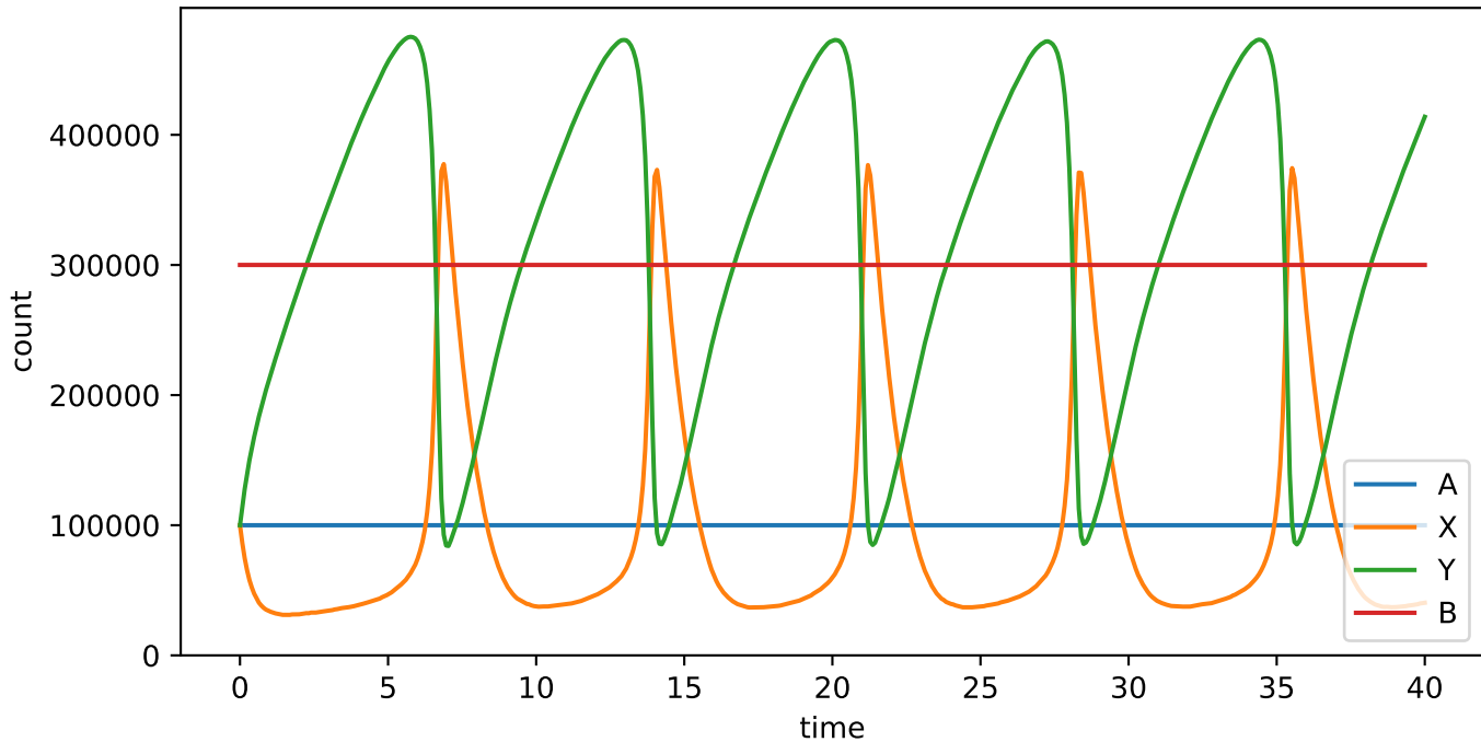
Order-3 Brusselator: batss, n=10^5
